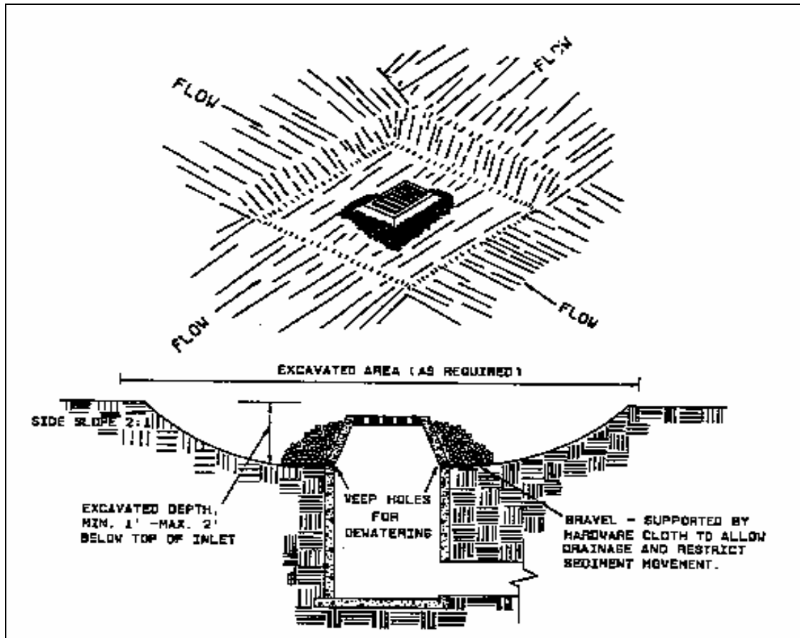
Figure 3.20. Excavated drop inlet protection (Source: Department of Civil, Construction, and Environmental Engineering, Iowa State University)
